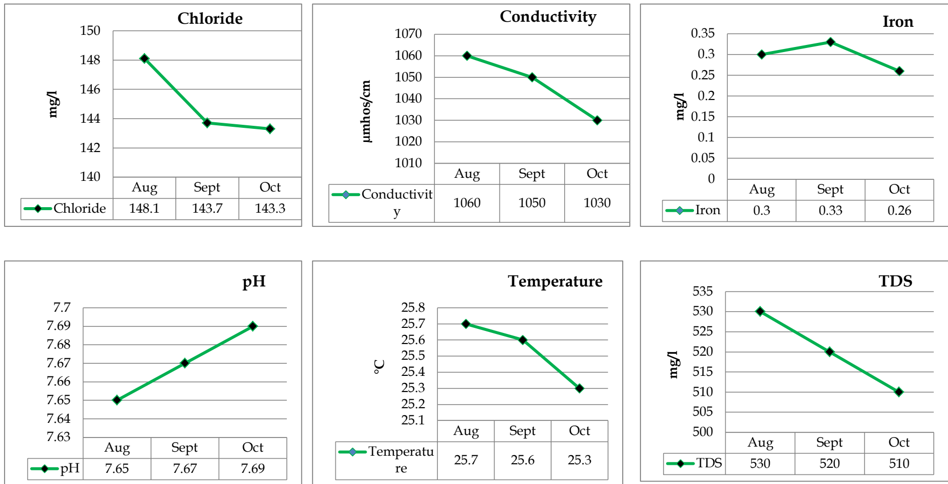
Figure 4-11: Summary of the Surface Water (GW2) August to October 2019
