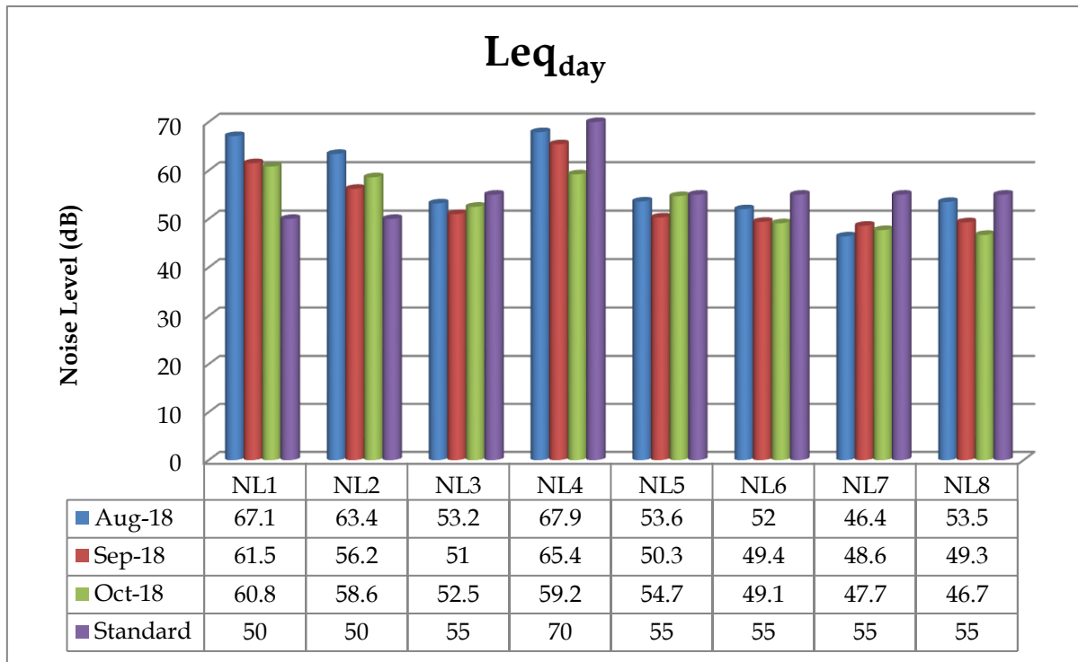
Figure 4-6: Summary of the ambient noise recorded at day time in August - October, 2019
