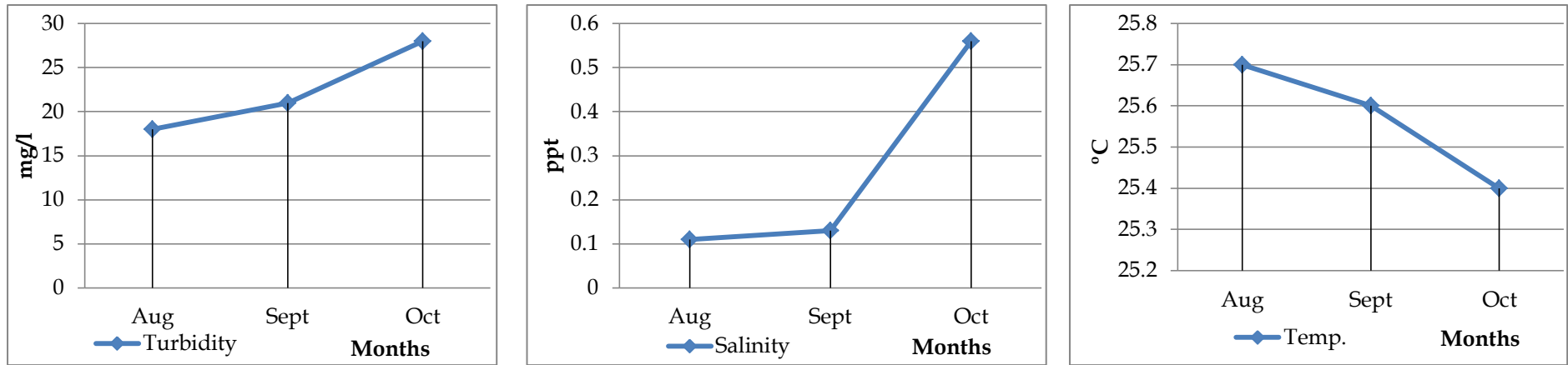
Figure 4-8: Summary of the Surface Water (SW1) August to October 2019
