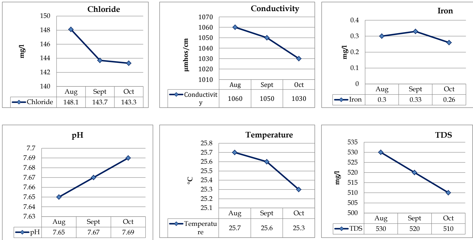
Figure 4-10: Summary of the Surface Water (GW1) August to October 2019
