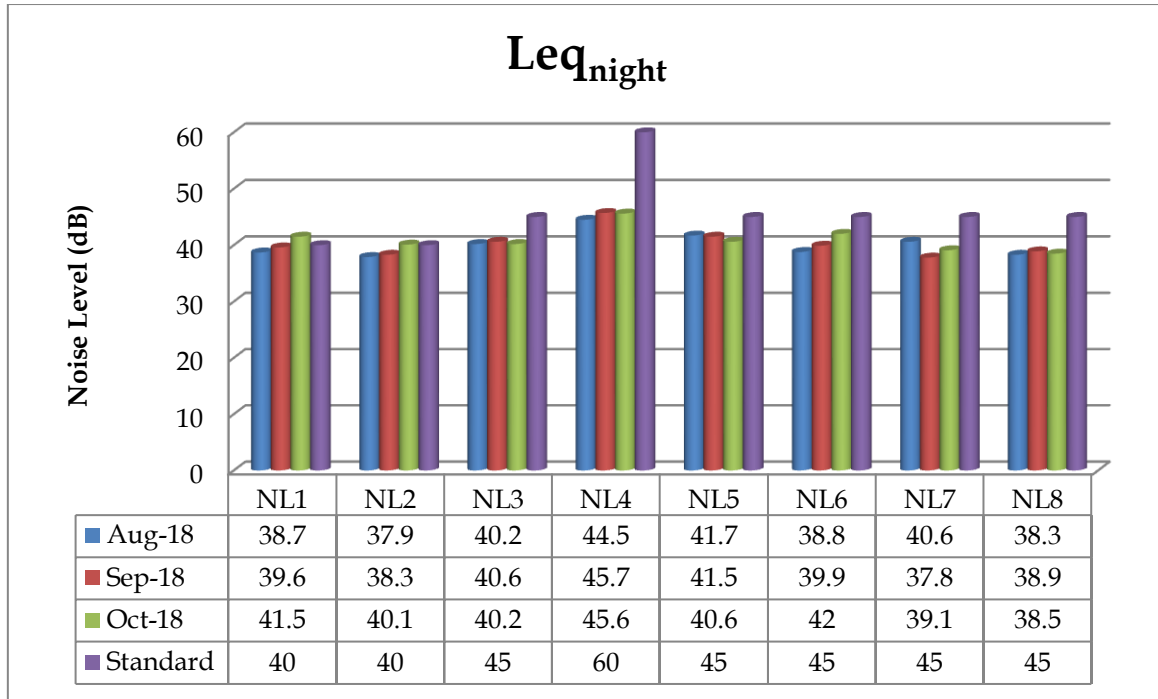
Figure 4-7: Summary of the ambient noise recorded at night time in August-October, 2019
