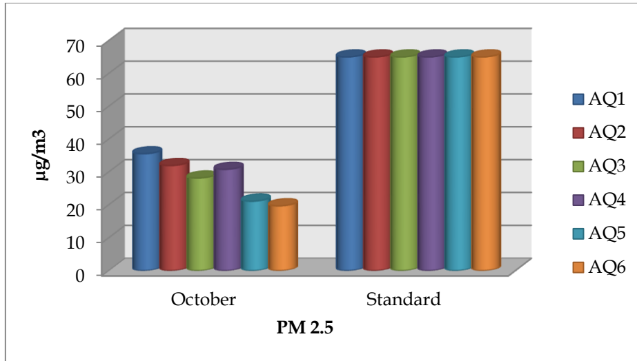
Figure 4-1: PM 2.5 Data Representation With Standard
